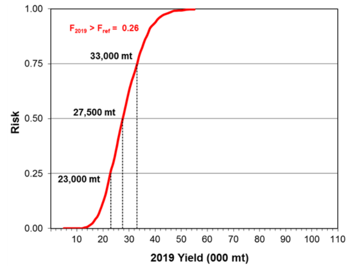
Figure 8. 2019 sensitivity ( \rho adjusted) yield projection risks for EGB haddock assuming 2018 catch at F_{ref} .
