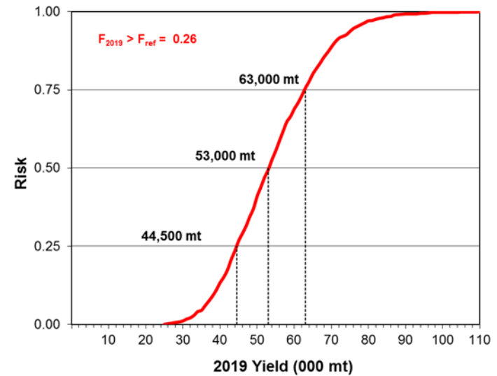
Figure 6. 2019 yield projection risks for EGB haddock assuming 2018 catch at F_{ref} .
