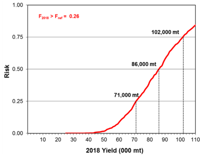
Figure 5. 2018 yield projection risks for EGB haddock.
