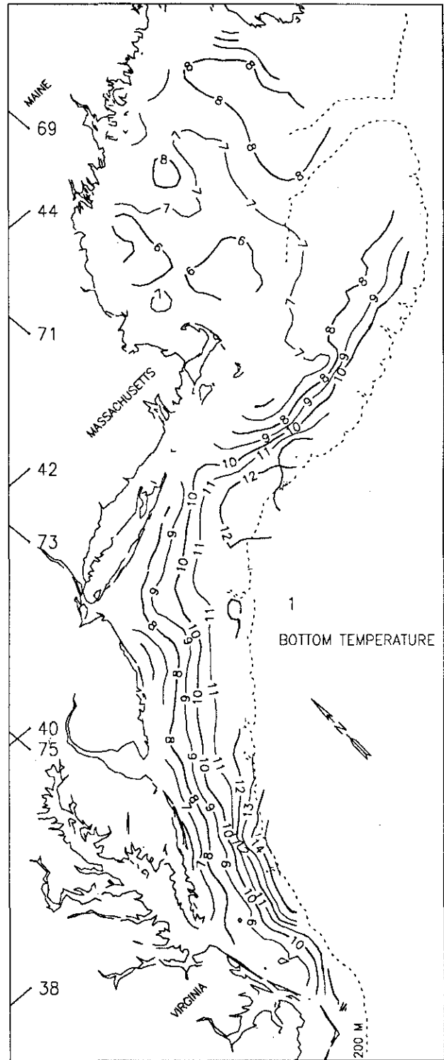
Figure 3. Expected (a) surface and (b) bottom temperature ( ^{\circ}\text{C} ) for January 1. The large numbers above the legend indicate the Julian day.
