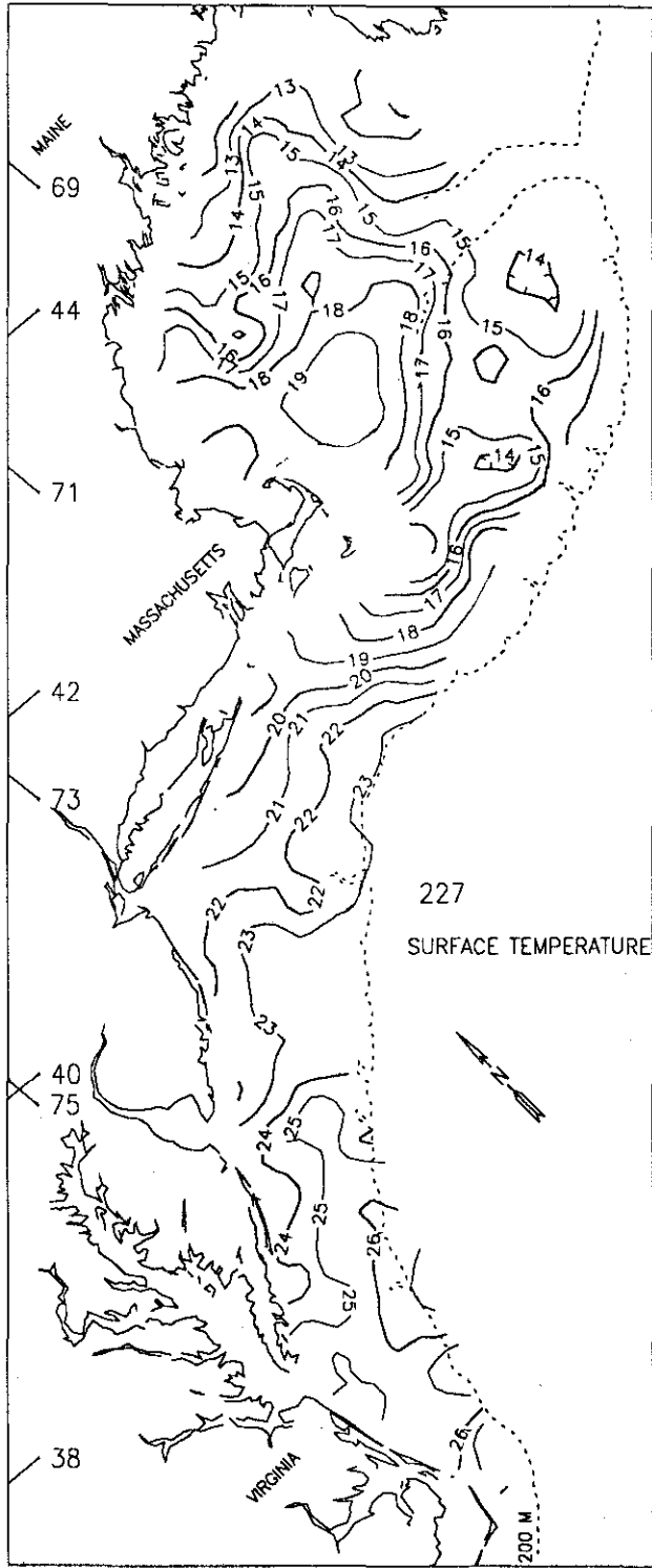
Figure 18. Expected (a) surface and (b) bottom temperature ( ^{\circ}\text{C} ) for August 15. The large numbers above the legend indicate the Julian day.
