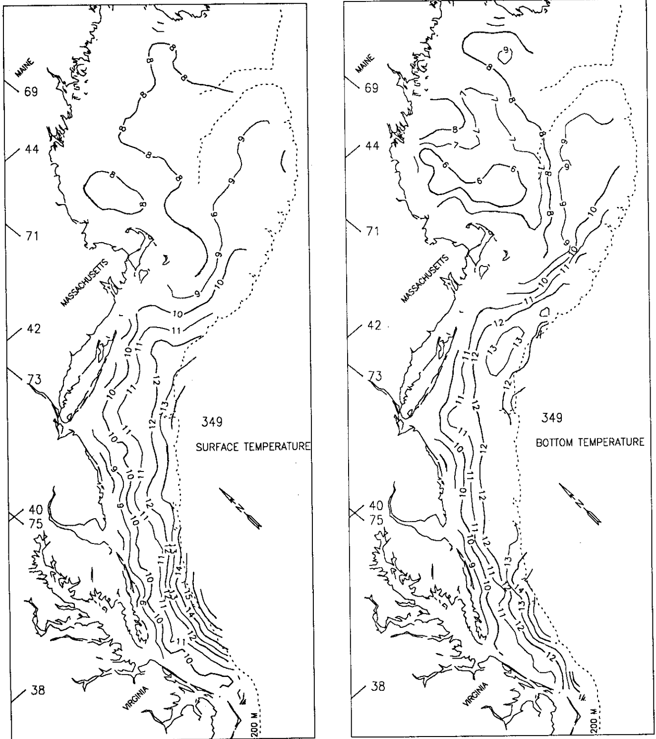
Figure 26. Expected (a) surface and (b) bottom temperature ( ^{\circ} C) for December 15. The large numbers above the legend indicate the Julian day.
