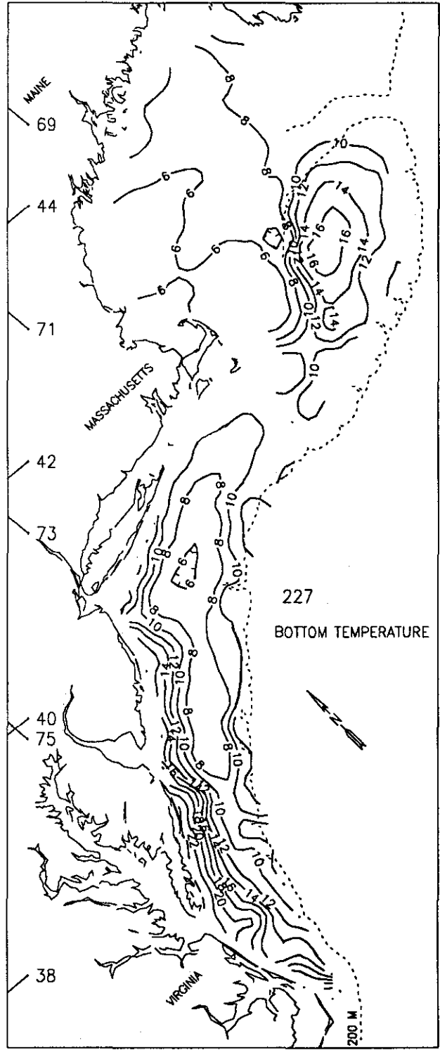
Figure 18. Expected (a) surface and (b) bottom temperature ( ^{\circ}\text{C} ) for August 15. The large numbers above the legend indicate the Julian day.
