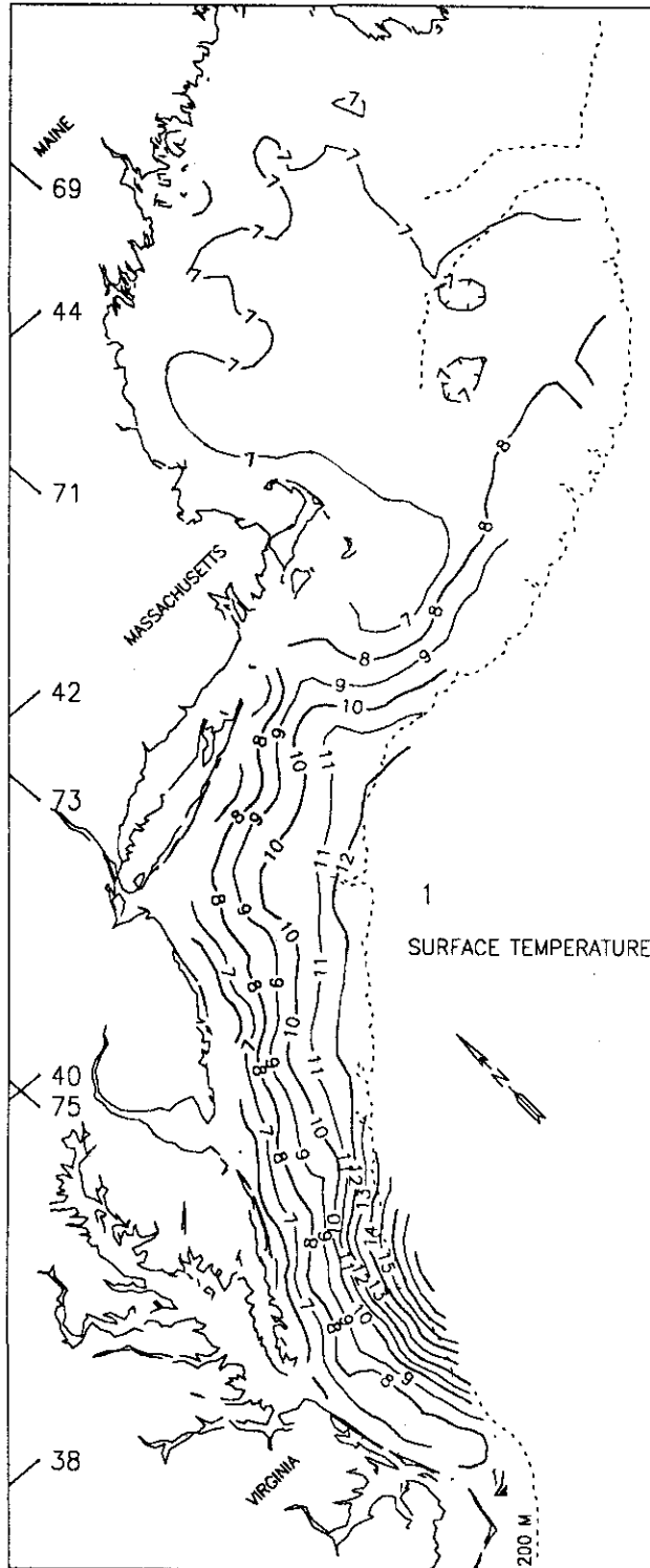
Figure 3. Expected (a) surface and (b) bottom temperature ( ^{\circ}\text{C} ) for January 1. The large numbers above the legend indicate the Julian day.
